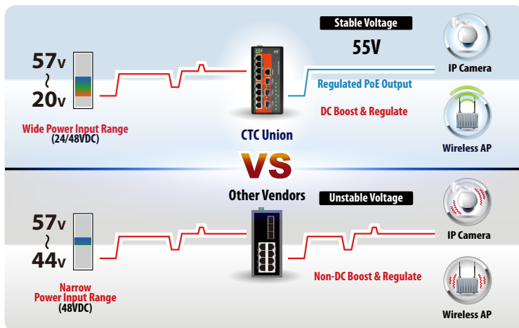
Figure 2 : Very high efficiency boost technology for PoE
