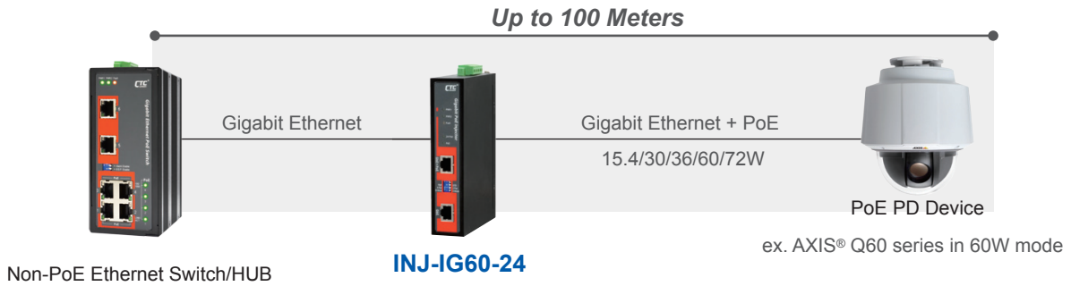
Figure 1 : INJ-IG60-24 Gigabit Ethernet PoE Injector
