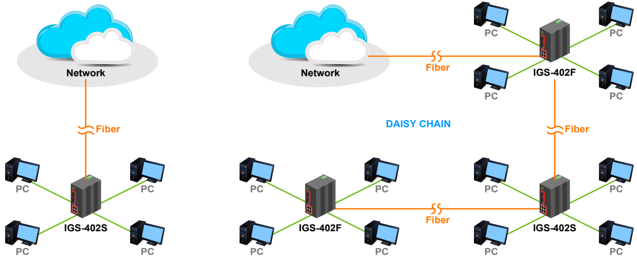
Figure 1 : IGS-402S & IGS-402F Gigabit Ethernet Switch Transmission
