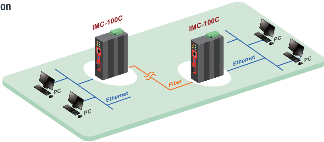
Figure 1 : IMC-100C Media Converter Transmission
