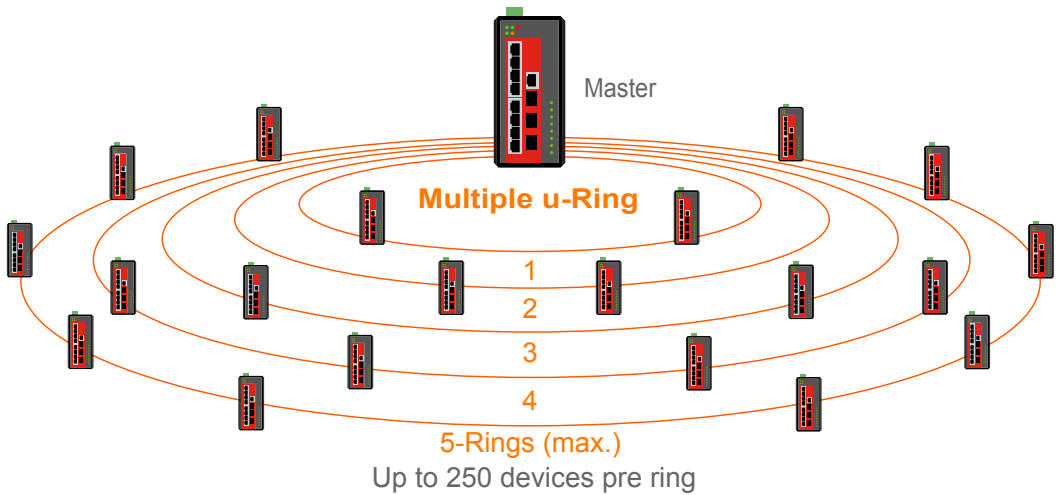
► Figure 5 : Multiple \mu -Ring
