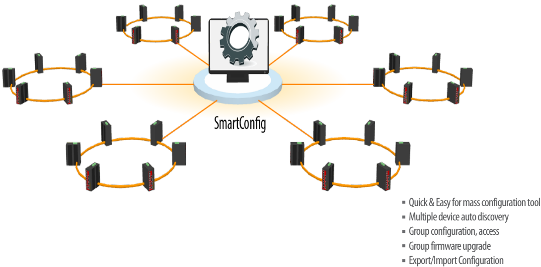
► Figure 5 : Multiple \mu -Ring
