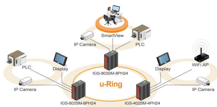
Figure 1 : Application Example
